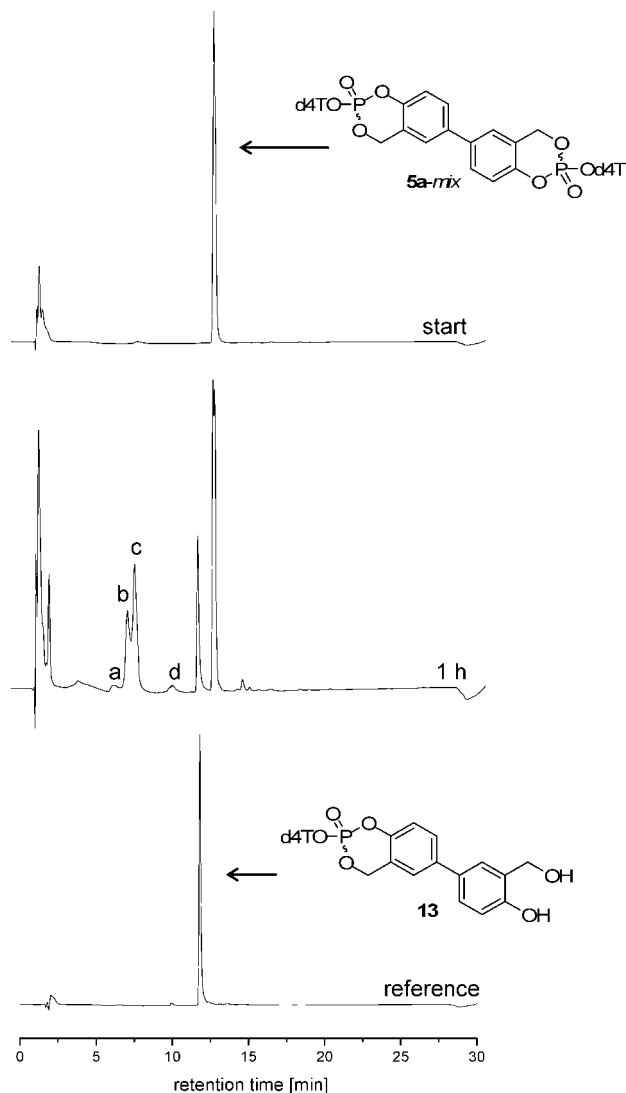
Figure 2. HPLC analytical proof of the formation of 13 during the hydrolysis of 5a-mix .
