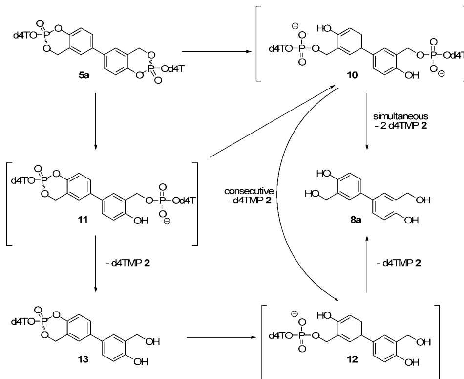
Scheme 3. Theoretical Pathways of Chemical Hydrolysis of 5,5'-Bis-(cycloSal-d4TMP) 5a
