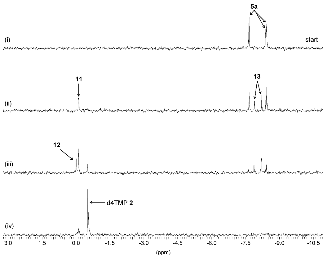
Figure 4. ^{31}\text{P} NMR hydrolysis study of 5a-mix .
