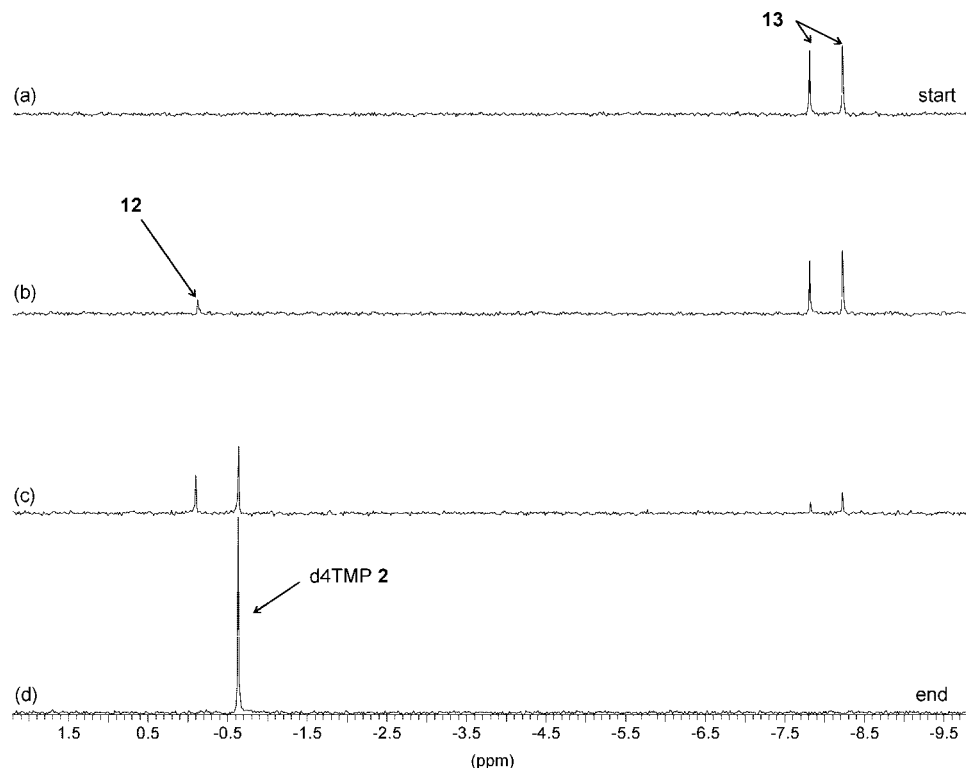
Figure 3. ^{31}\text{P} NMR hydrolysis study of 13 (diastereomeric mixture).
