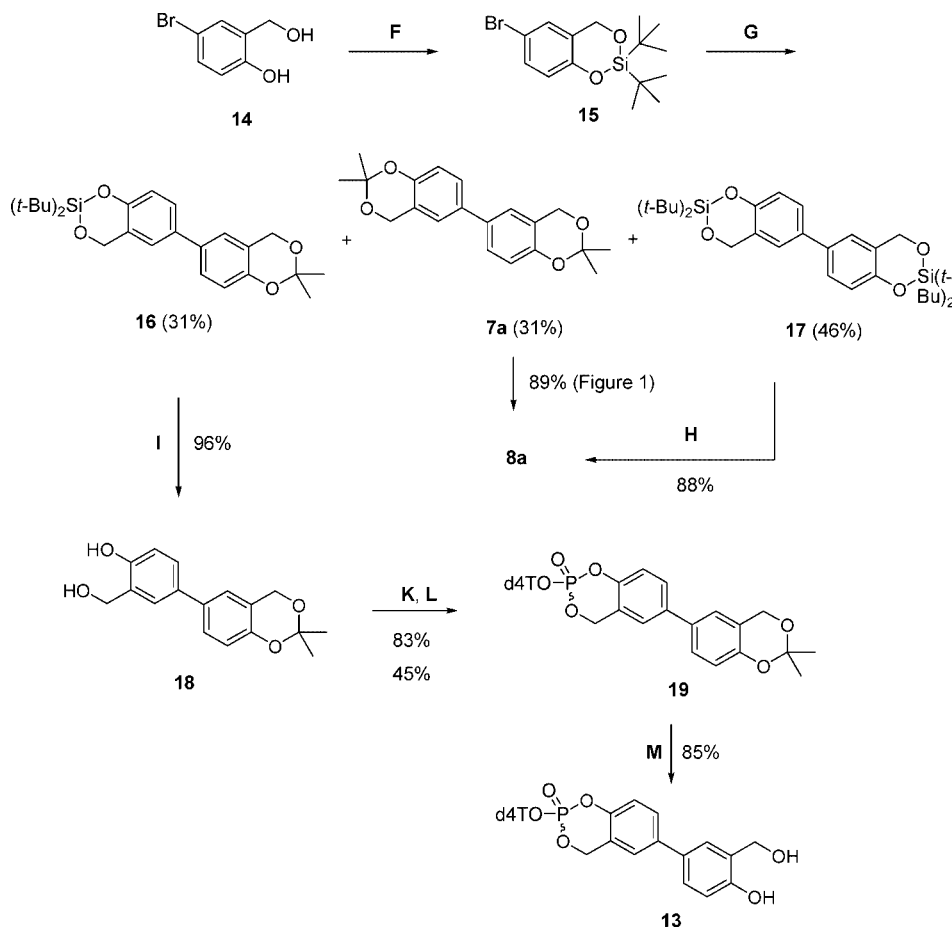
Scheme 4. Synthesis of 4,7- O -di- tert -Butylsilyl-4',7'- O -isopropylidene-3,3'-bis(hydroxymethyl)biphenyl-4,4'-diol 16 and 5-(Saligen-5'-yl)- cycloSal -d4TMP 13 a
