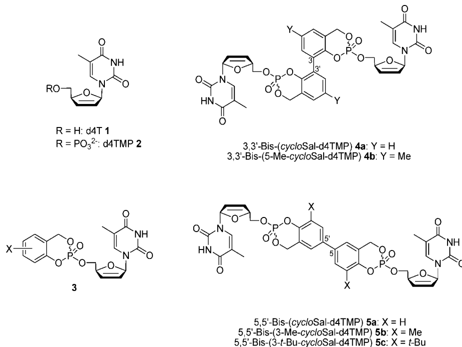
Figure 1. Structures of d4T 1 , d4TMP 2 , “monomeric” cycloSal-d4TMP 3 , and bis-(cycloSal-d4TMP)s 4 and 5 .
